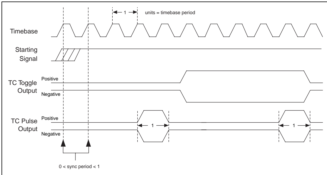
Figure 1-2. MIO Device Counter Timing and Output Types
